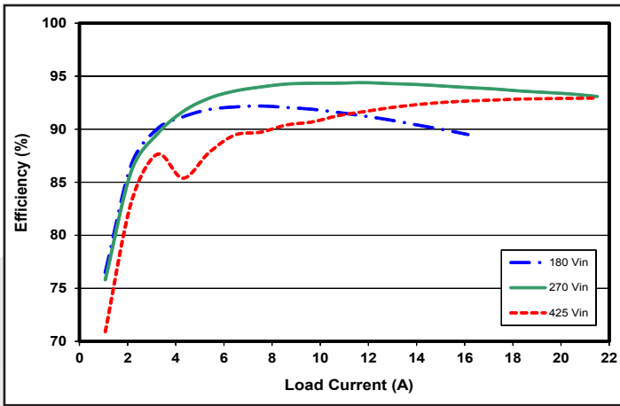
Figure 1: Efficiency at nominal output voltage (28V) vs. load current for three input voltage at 25°C.
